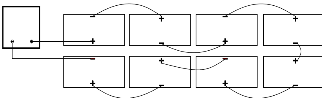
Fig. 5-4 Split J-Box at module middle position for horizontal direction
